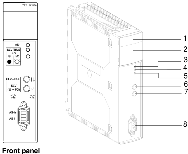
Front panel
