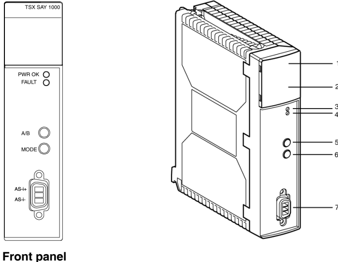
Front panel
